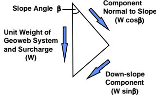
Figure 4 Stability Analysis of the Geoweb Slope Protection System
