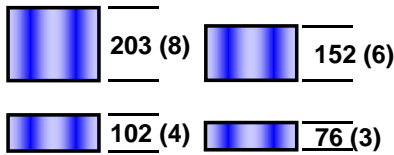
Figure 2 Geoweb Cell Size and Depth
