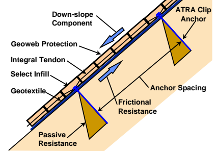
Figure 4 Stability Analysis of the Geoweb Slope Protection System
