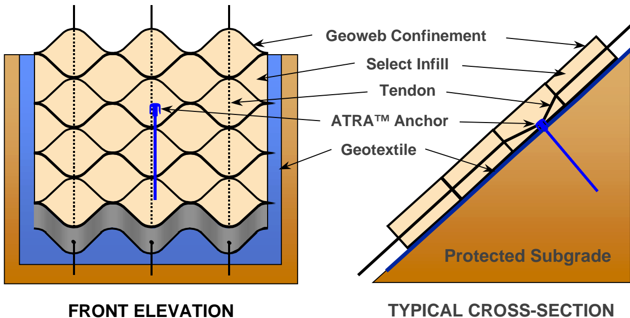
Figure 1 Key Components of the Geoweb System
