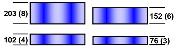
Figure 2 Geoweb Cell Size and Depth
