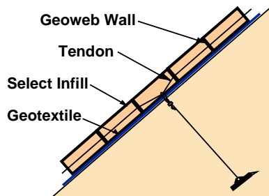
Figure 3 Typical Geoweb Anchorage Schemes
