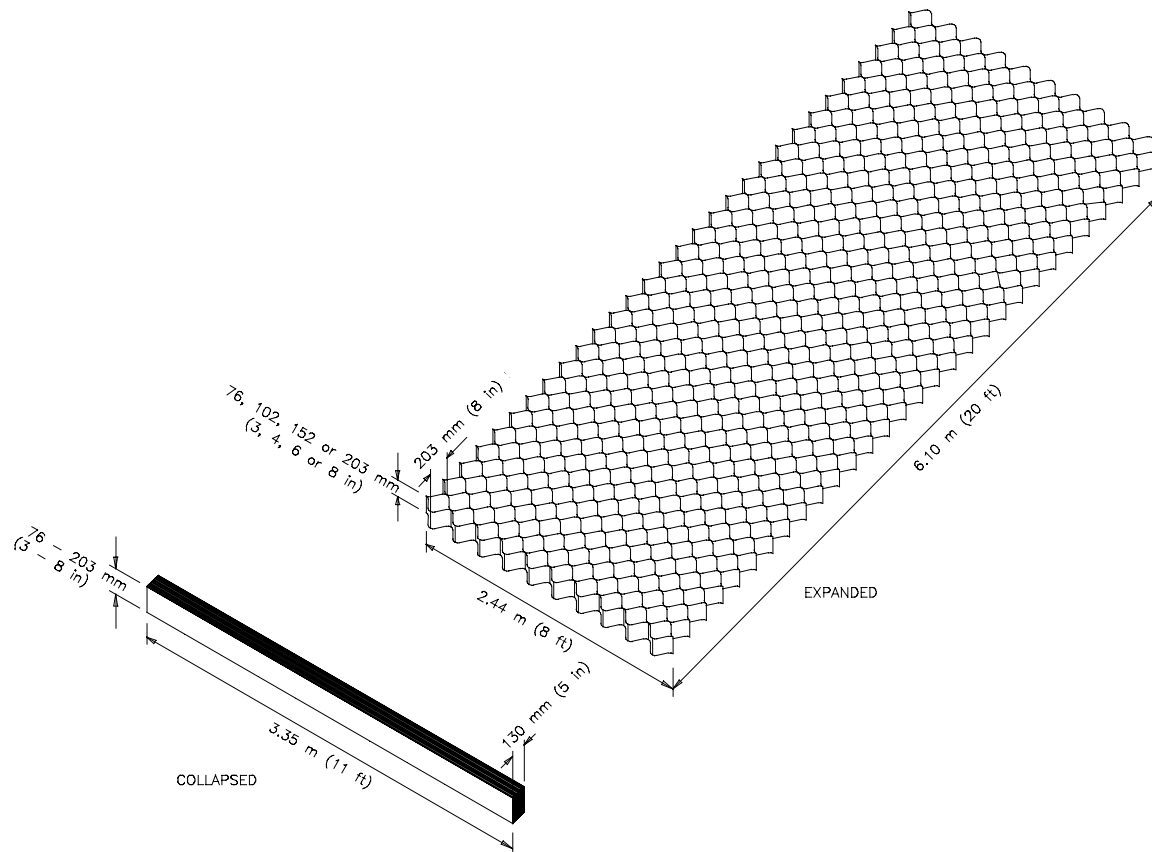
Figure 1 Standard Geoweb Sections
