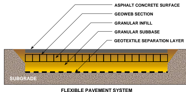
Figure 2 Flexible Pavement Detail
